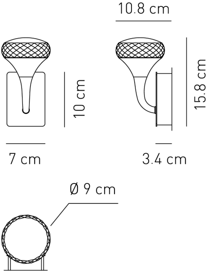
Product Dimensions
