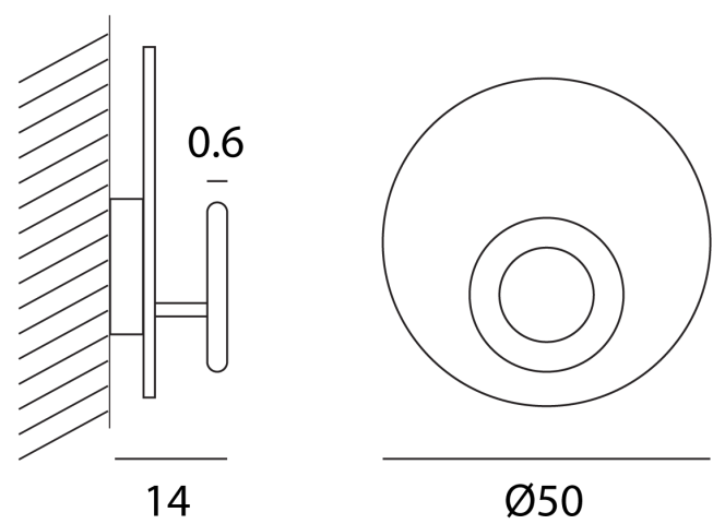
Product Dimensions
