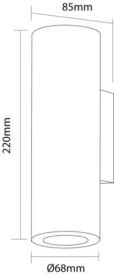
Product Dimensions
