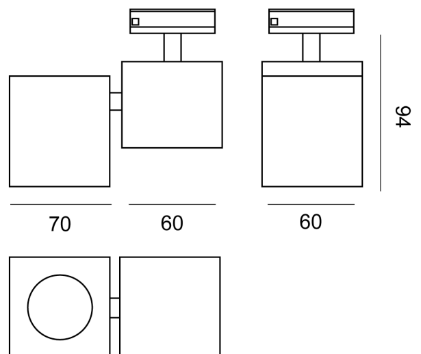
Product Dimensions
