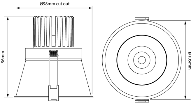
Product Dimensions
