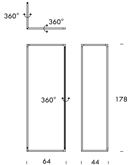
Product Dimensions
