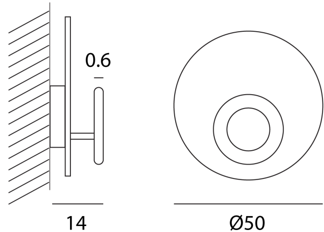
Product Dimensions
