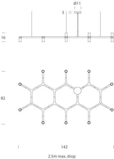
Product Dimensions
