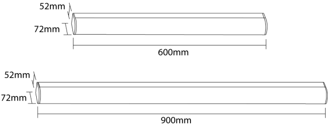
Product Dimensions
