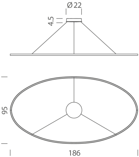
Product Dimensions
