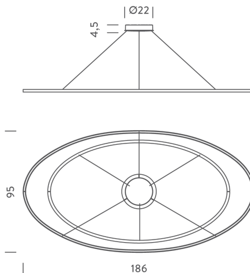
Product Dimensions
