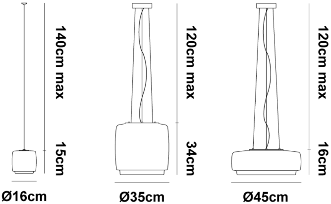
Product Dimensions
