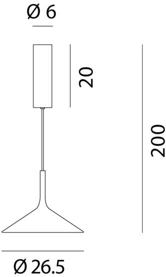
Product Dimensions
