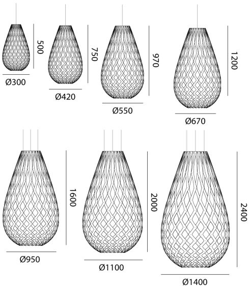
Product Dimensions
