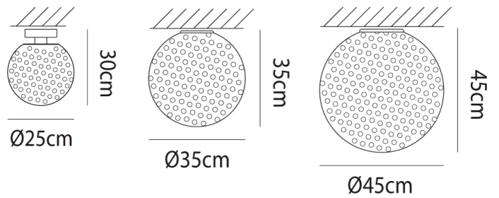
Product Dimensions
