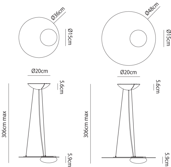
Product Dimensions
