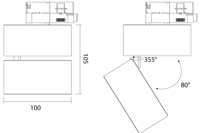
Product Dimensions
