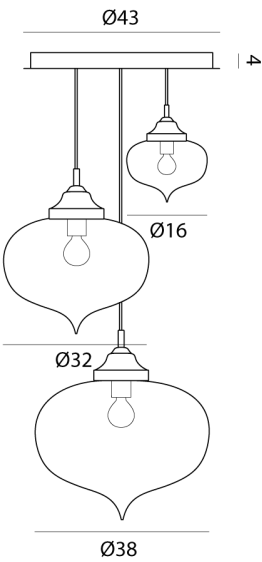
Product Dimensions
