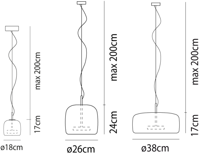
Product Dimensions
