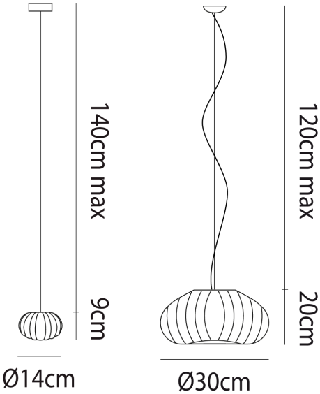
Product Dimensions
