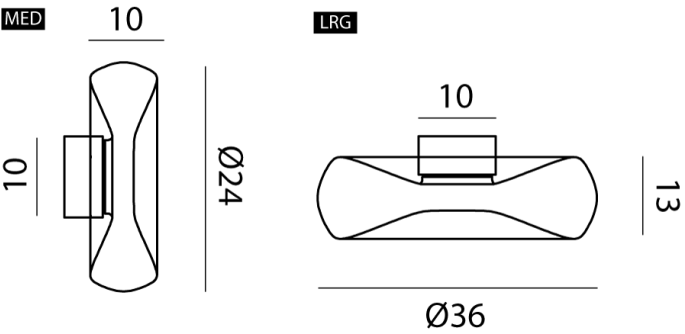
Product Dimensions
