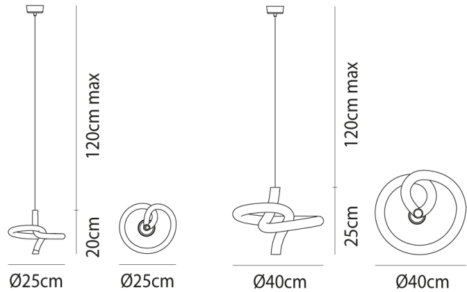
Product Dimensions
