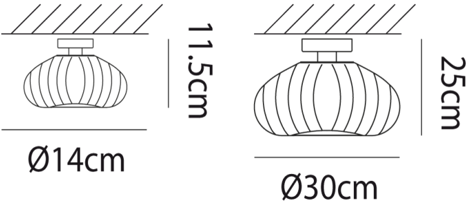
Product Dimensions
