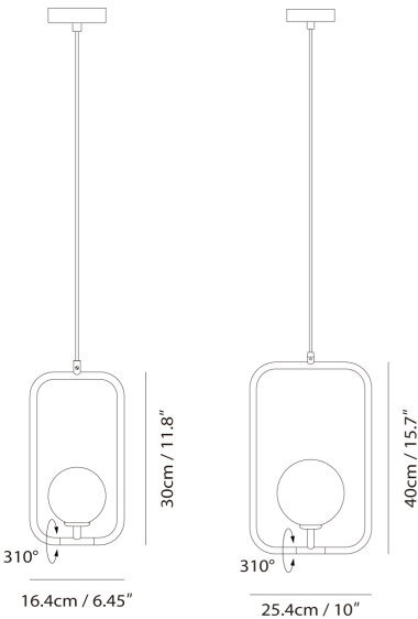
Product Dimensions
