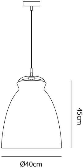
Product Dimensions
