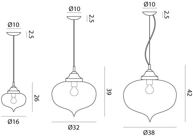
Product Dimensions
