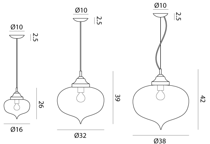
Product Dimensions
