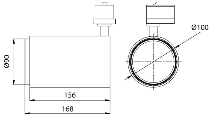
Product Dimensions
