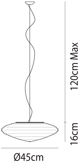
Product Dimensions
