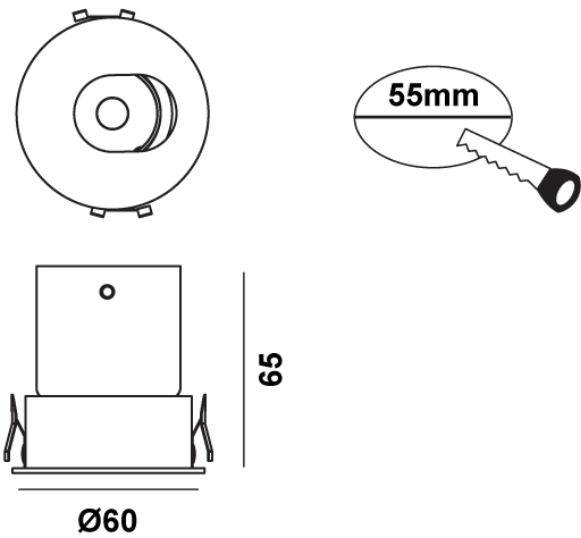
Product Dimensions
