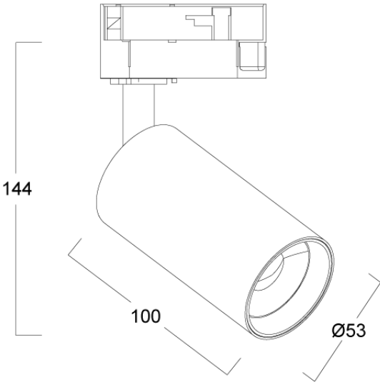
Product Dimensions
