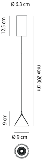
Product Dimensions
