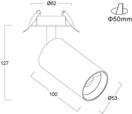
Product Dimensions
