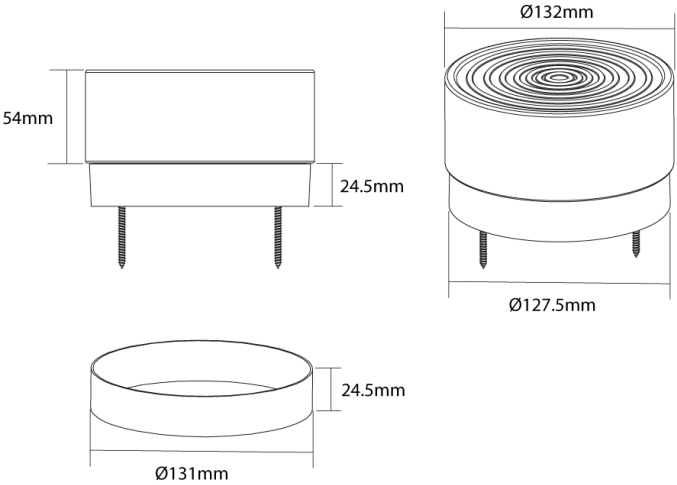
Product Dimensions
