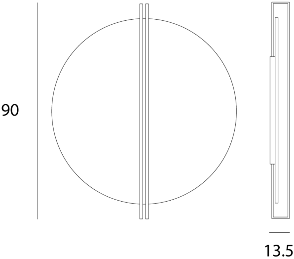
Product Dimensions
