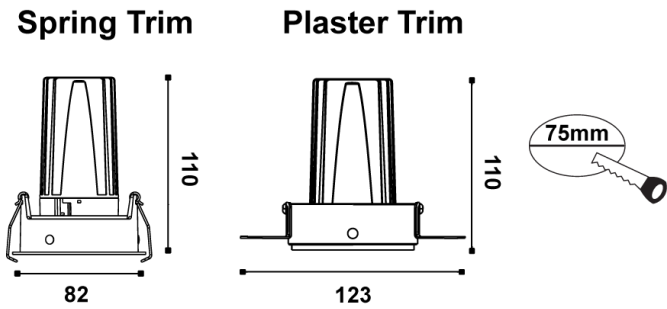
Product Dimensions
