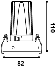
Spring Trim
