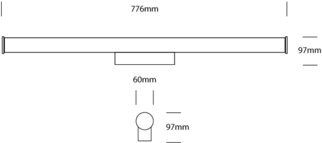
Product Dimensions
