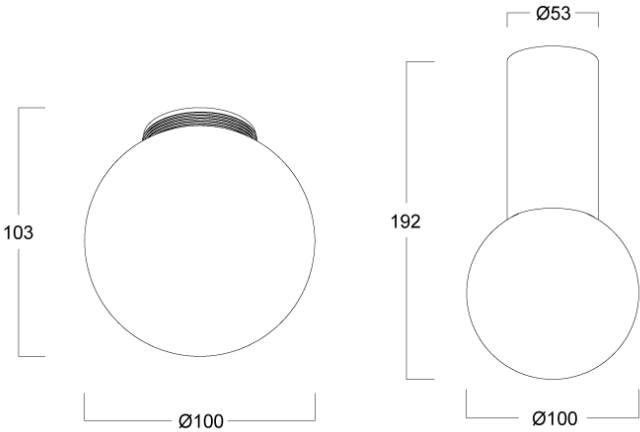
Product Dimensions
