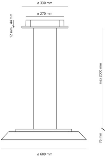
Product Dimensions
