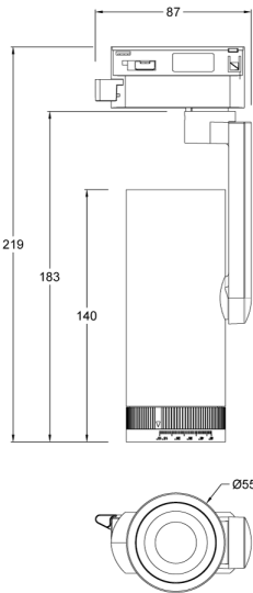
Product Dimensions
