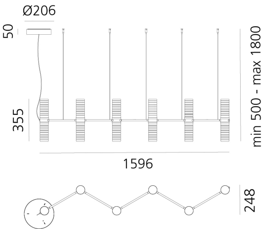
Product Dimensions
