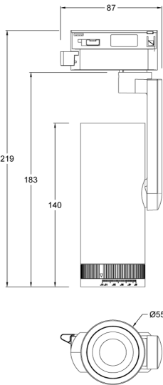
Product Dimensions
