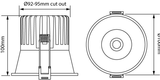
Product Dimensions
