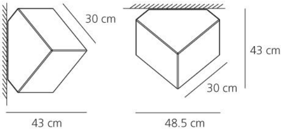
Product Dimensions
