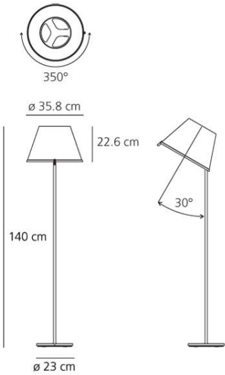
Product Dimensions
