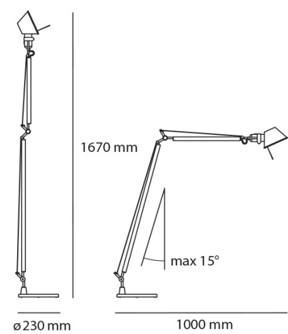
Product Dimensions
