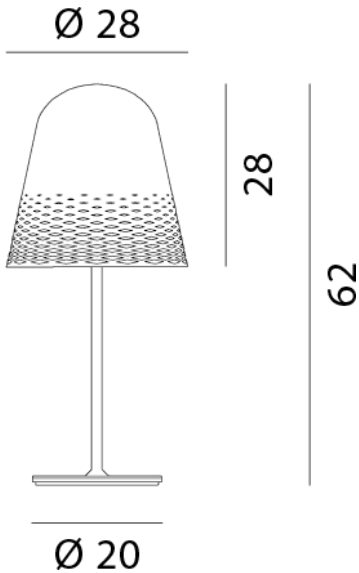
Product Dimensions
