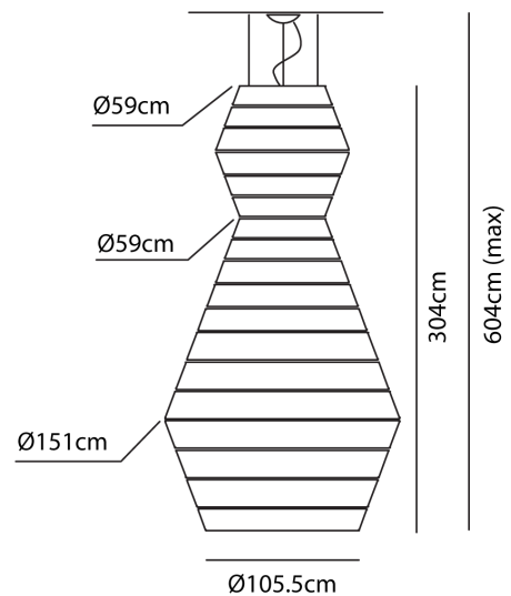
Product Dimensions
