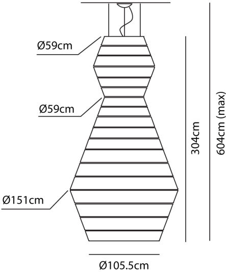
Product Dimensions
