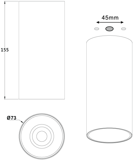
Product Dimensions
