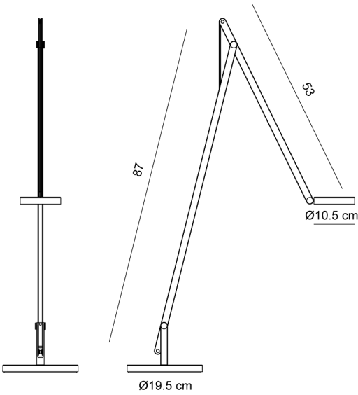
Product Dimensions
